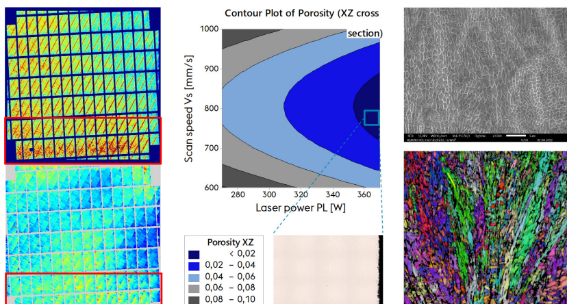
Left: Optimisation goal "build zone" detected by process monitoring using EOSTATE Exposure OT (top) and EOSTATE MeltPool (below).
