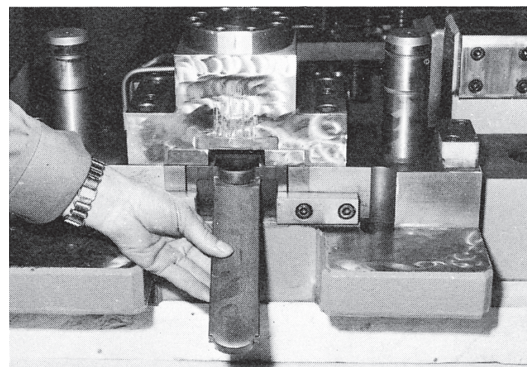
Cold cropping tool made from Uddeholm Viking.
