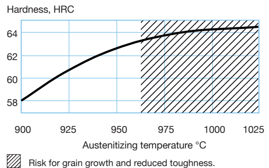
Hardness and retained austenite as a function of austenitizing temperature.
