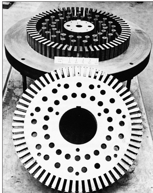
Uddeholm Sverker 3 blanking and piercing tool to produce lamination plates from abrasive high-silicon sheet.
