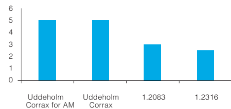
Uddeholm Corrax for additive manufacturing has excellent corrosion resistance, fully matching the conventionally manufactured Corrax and better than the corrosion resistant standard grades used for plastic moulding.
