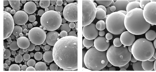
The process and quality control in Uddeholm's powder lab is your reliable guarantee for homogeneity in size and shape. The result is powder with minimal cladding.
