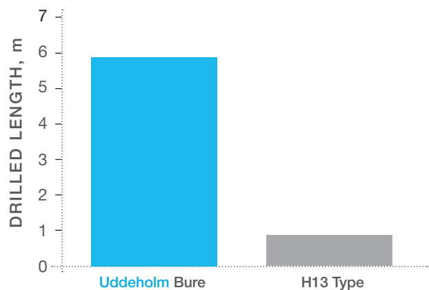
GUN-DRILLING OF COOLING CHANNELS IN SOFT ANNEALED MATERIAL
