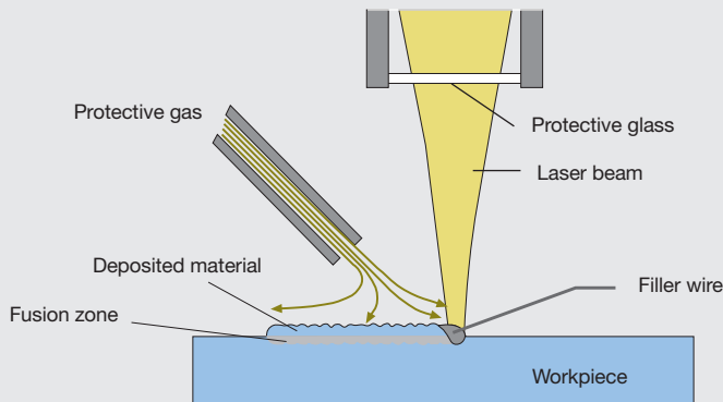
Fig. 3 Laser Welding
