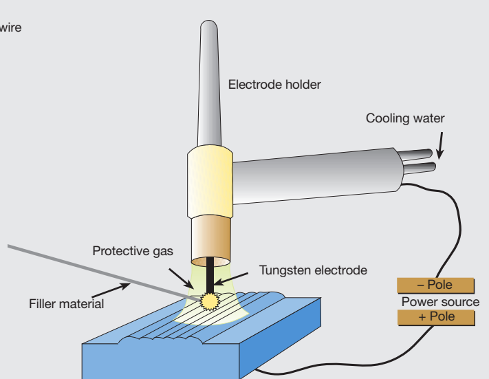
Fig. 2 Gas Tungsten Arc Welding GTAW (TIG)
