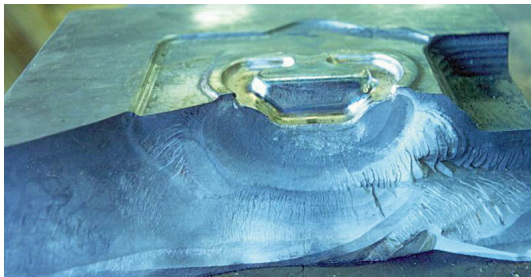
Totally cracked die.
