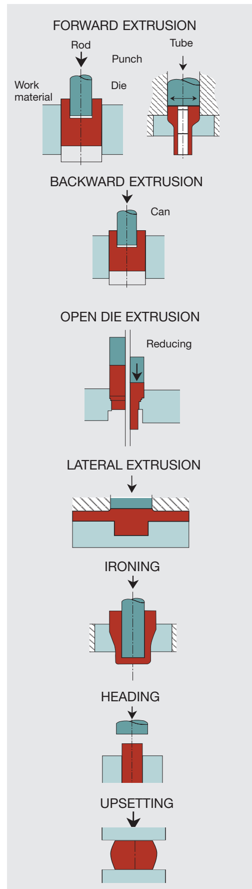
Typical processes in warm forging.
