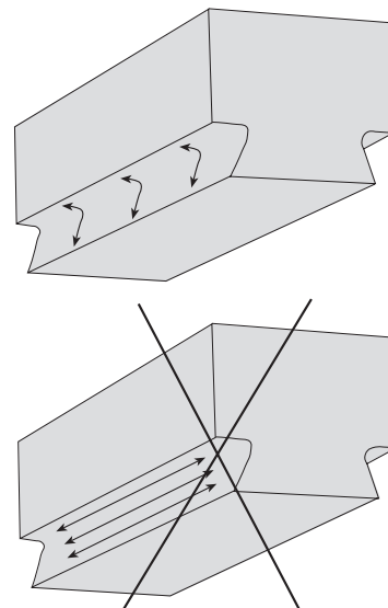
Grinding of dove-tail radii.
