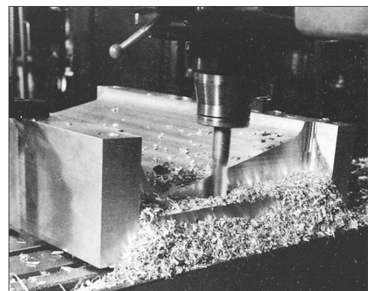
Milling Alumec 89.
